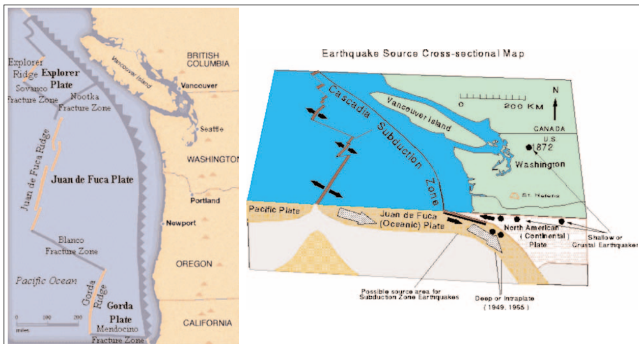
Figure 6. Cascadia Subduction Zone in map view and cross section.
