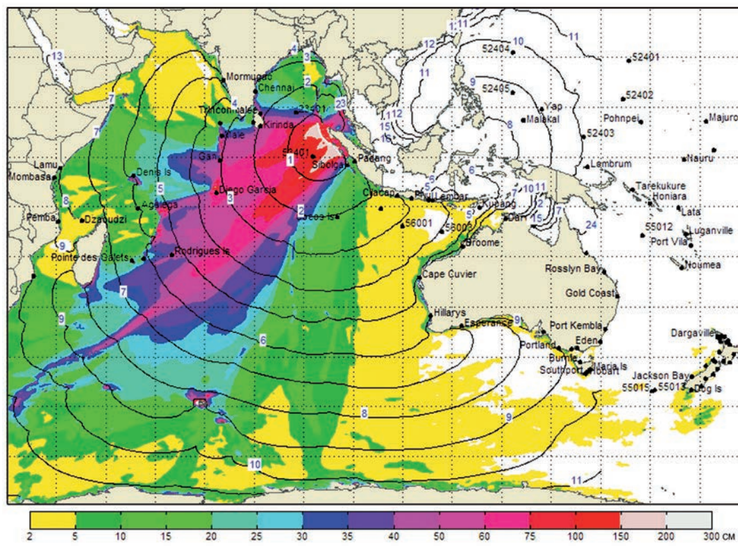
IO-TWS RTSP Australia tsunami threat map for the Indian Ocean from the 26 December 2004 M9.1 earthquake off Sumatra, Indonesia. This forecast would have been issued if there had been international warning centres in operation in 2004. Colour bands show tsunami energy propagation directions and maximum offshore amplitudes. Expected tsunami travel time contours are shown at 1-hr intervals. Courtesy of Joint Australia Tsunami Warning Centre.
